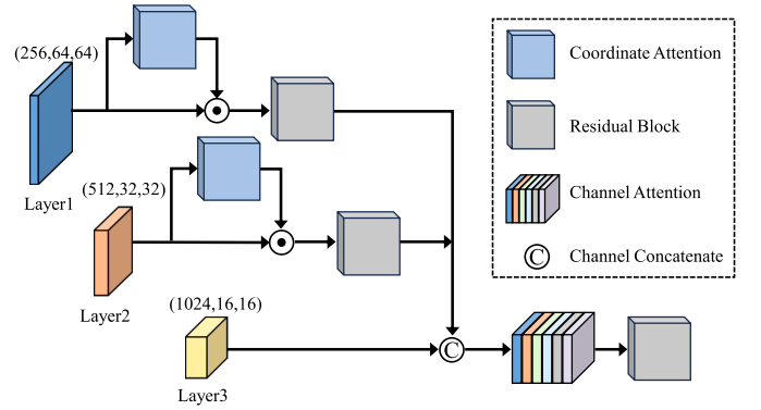
Fig. 5. Illustration of MFF.
