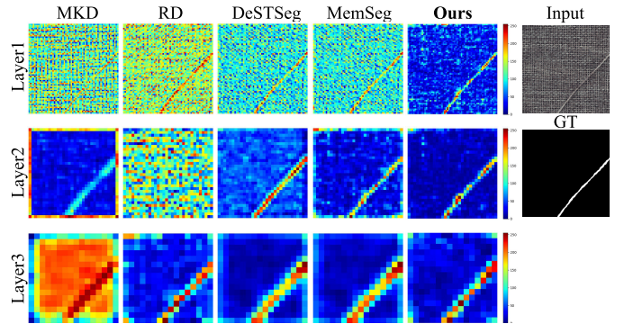
Fig. 9. Visualization of features. The images are captured from feature layers of our frozen teacher model or other feature extraction models.
