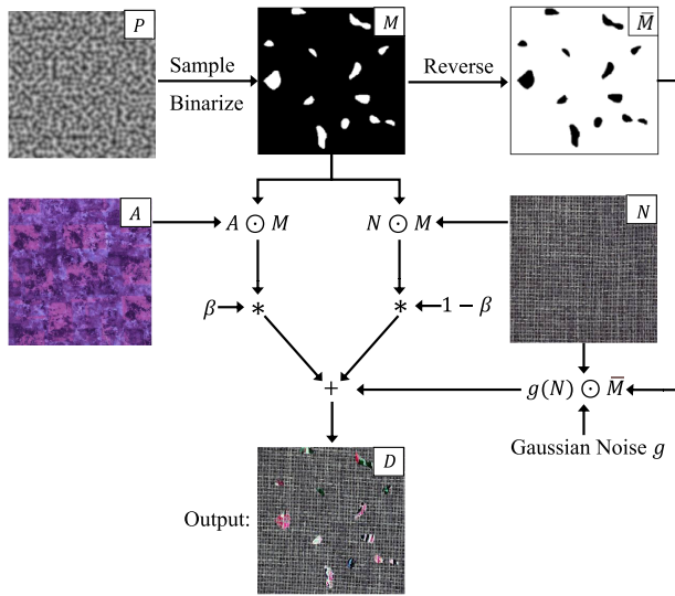
Fig. 3. Defect generation process. The binary anomaly mask M is generated from Perlin noise P . The defective regions are sampled from A according to M and placed on the normal image N to generate the anomalous image D .
