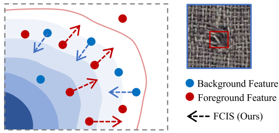
Fig. 1. Illustration of how textures affect the distribution of features. The foreground features (anomalies) are mixed with the background features (normal), making it difficult to distinguish. The proposed feature contrast interference suppression (FCIS) could enlarge the feature distance between foreground and background textures while suppressing the distribution of background features to obtain a more robust background representation.
