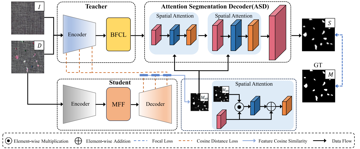
Fig. 2. Pipeline of the proposed method. First, pairs of normal images and pseudodefected images are input into the teacher model for BFCL. After BFCL training is completed, the teacher model weights are frozen for denoising knowledge distillation, which trains the student model to incorporate MFF. Finally, ASD training is performed using focal loss as the loss function.
